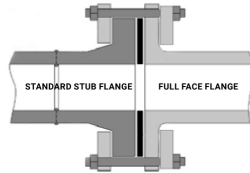
Bolt Arrangement: Full Face Flange
